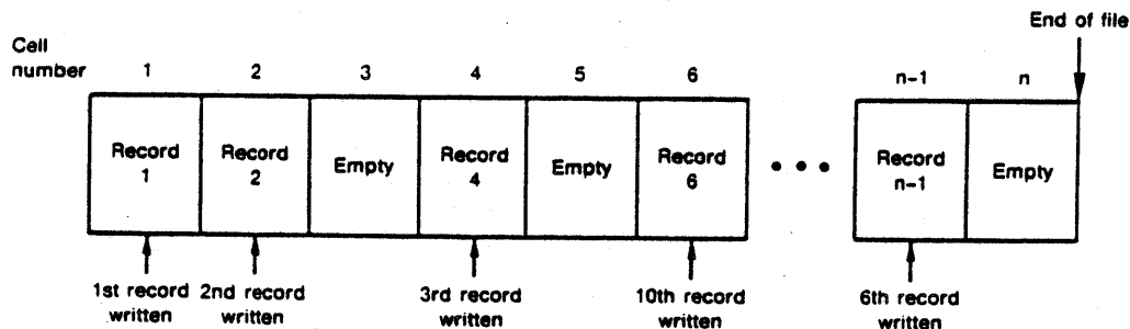
Figure 8: Relative File Organization
