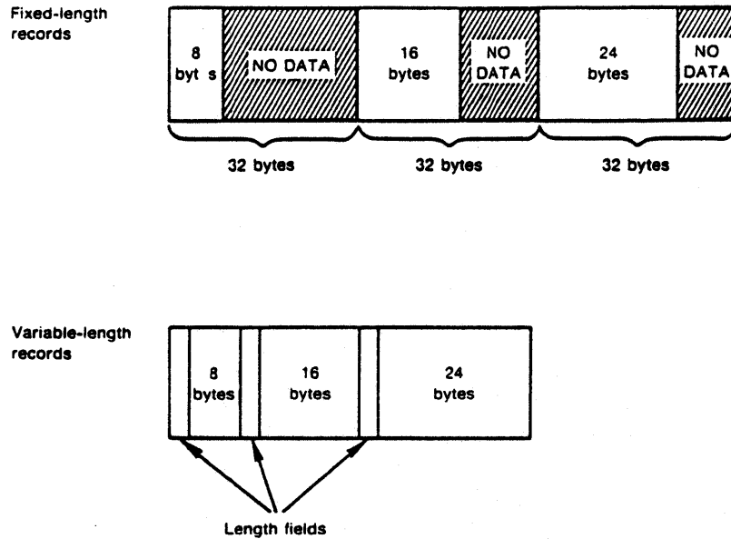
Figure 5: Fixed-Length and Variable-Length Record Formats
