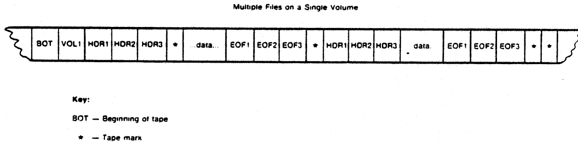
Figure 4: Magnetic Tape Structure
