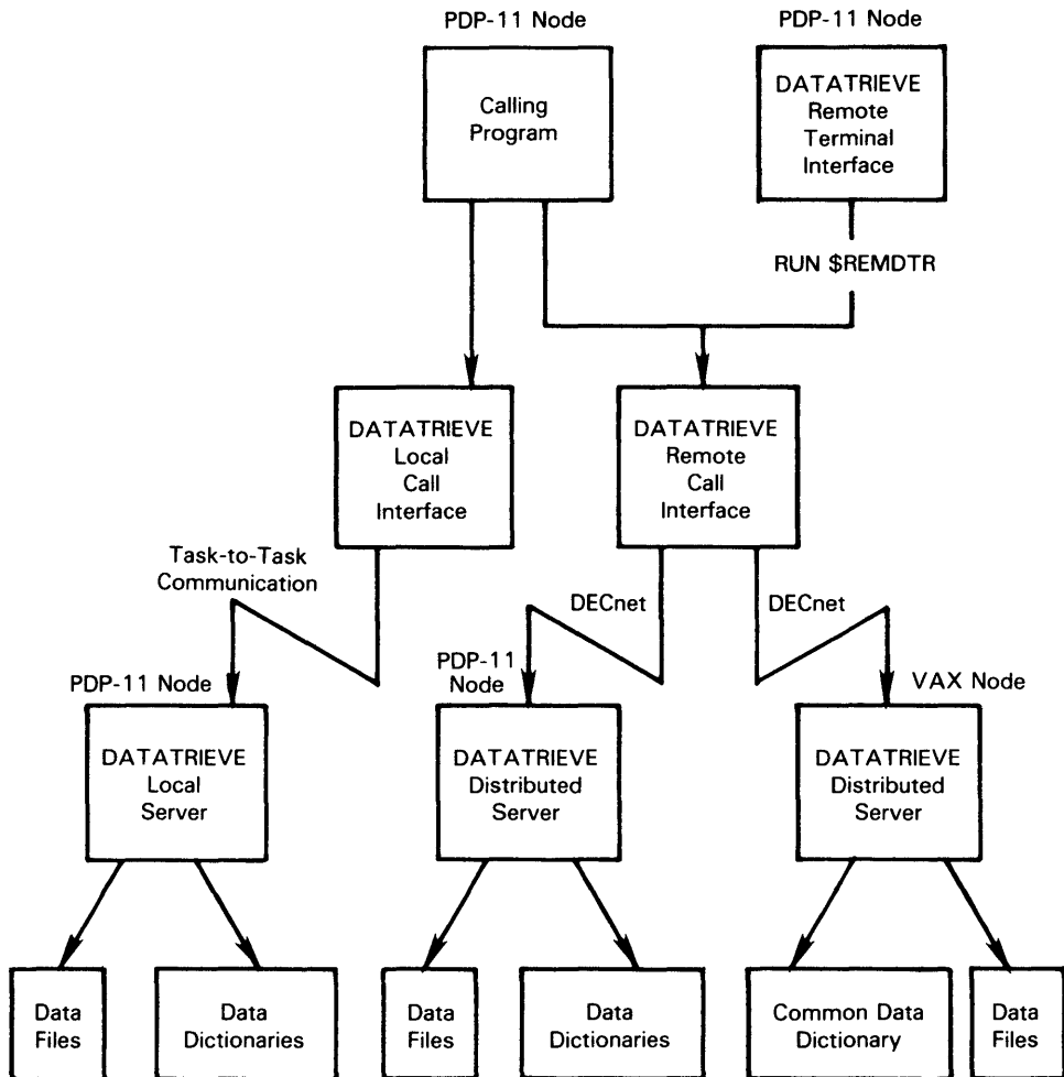
Figure 1-1: Distributed Data Access and Call Interface
