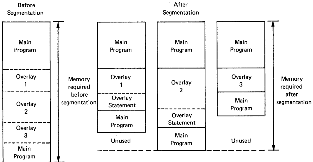
Figure 8-3 Segmenting a Program with the OVERLAY Statement
